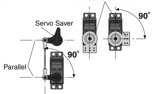
Direct Servo Saver Horn
